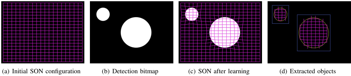
Fig. 1. Approach overview. The images show the different steps of our algorithm using a synthetic occupancy grid.
