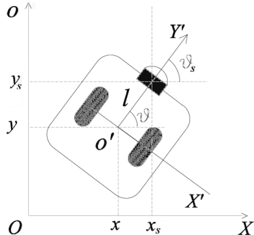
Fig. 1. Robot configuration.
