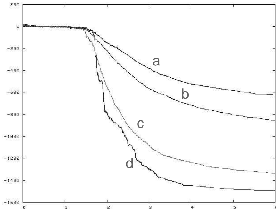
Figure 8: Trajectories associated with the cooling simulations described in table 1. The energy evolution is plotted as a function of the temperature ( x = -\log(T) , y = U ). Trajectories a , b , c have been obtained using geometrical schedules, while d corresponds to the proposed adaptive scheme.
