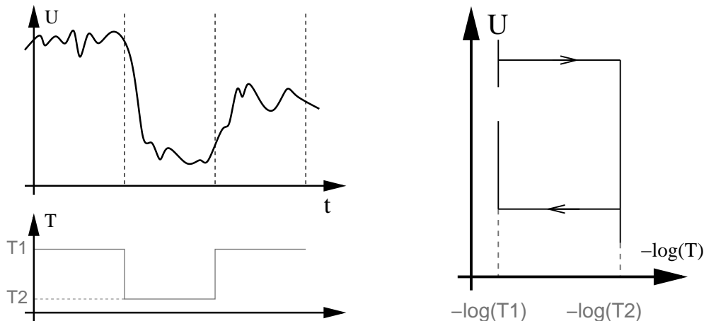
Figure 5: Theoretical illustration of the critical temperature phenomenon. When the system stays, even very shortly, under a specific temperature, the average energy brutally decreases.
