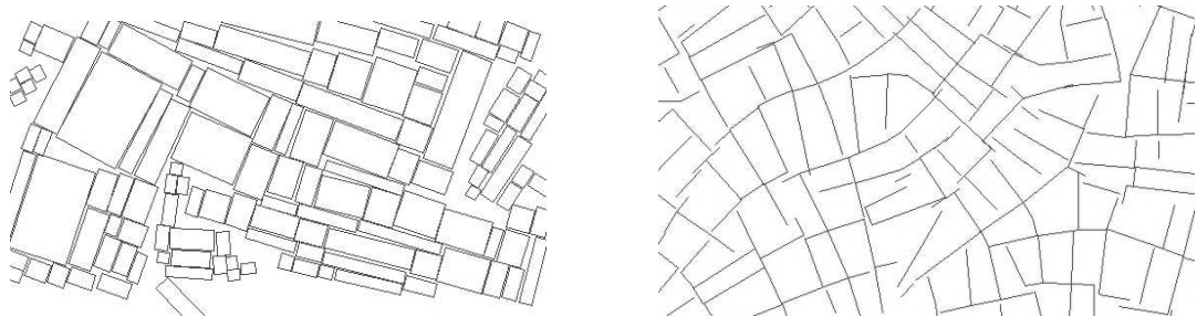
Figure 1: Simulation result showing the influence of the internal field on the process of rectangles and segments.
