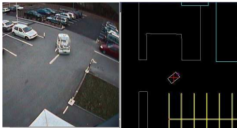
Fig. 15 The ParkView platform: left) camera view of the Cycab experimental car moving in the parking lot of the laboratory; right) the Cycab as detected on the tracking system.
