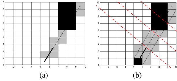
Fig. 3. Grey cells are searched for obstacles; black cells are occupied. A point of the robot and a cell are respectively considered in (a) and (b) image. The arrow is the considered relative velocity while the red dotted lines delimit searching areas for different times to collision.
