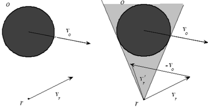
Fig. 2. Collision Cone for a punctual robot and a circular obstacle with linear velocity v_o ; v_r is in collision.
