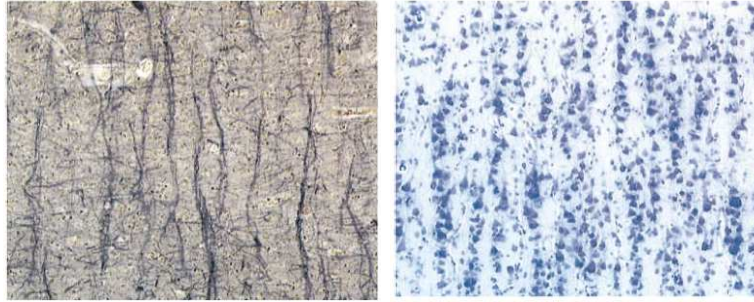
Figure 4: Myelinated fibre bundles (left) and cell soma aggregates (right) in the same cortical region. These observations suggest minicolumnar organization in the cortex (From [10]).
