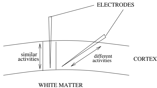
Figure 5: Mounca's pioneering experiment. When he moved an electrode perpendicular to the cortex surface, he encountered neurons with similar electrical activities while moving the electrode obliquely gave him different types of recordings. So he showed the existence of 300-500 \mu\text{m} wide columns in the cortex.
