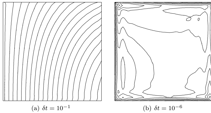
Figure 4: Pressure contour lines with \mathbb{P}_2/\mathbb{P}_2 finite elements in a 40 \times 40 mesh: \mathbf{u}_h^0 = I_h^2 \mathbf{u}_0
