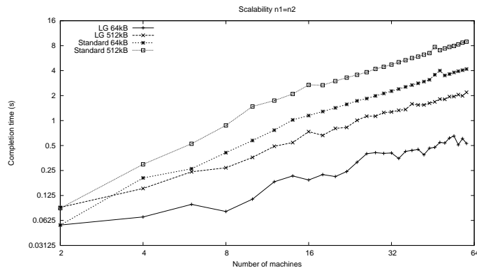
Fig. 5. Performance of the algorithms when varying the number of processes with n_1 = n_2
