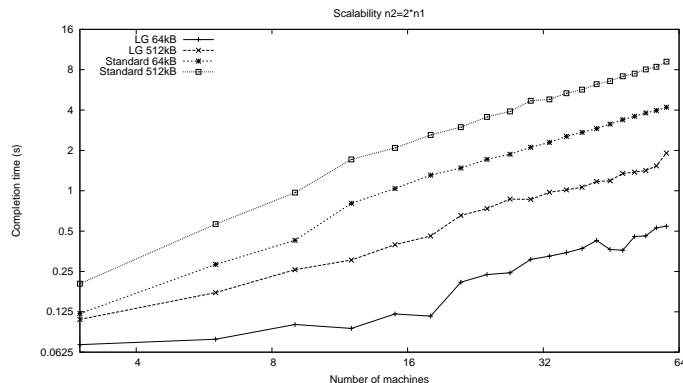
Fig. 6. Performance of the algorithms when varying the number of processes with n_2 = 2 \times n_1
