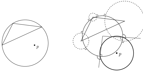
Figure 1: A cell in conflict in Delaunay triangulation (left) and regular triangulation (right)
