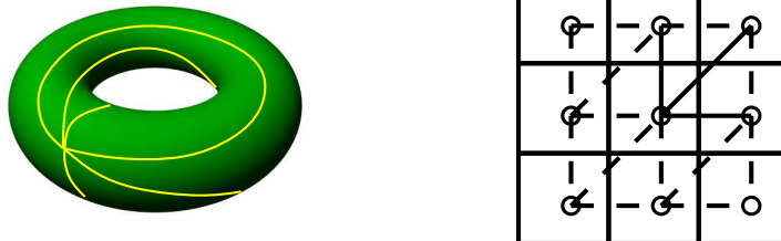
Figure 8: Left: invalid triangulation of \mathbb{T}^2 with a single vertex. Right: 9 periodic copies are shown.
