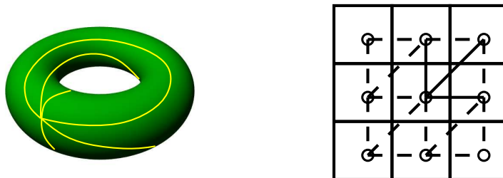
Figure 8: Left: invalid triangulation of \mathbb{T}^2 with a single vertex. Right: 9 periodic copies are shown.
