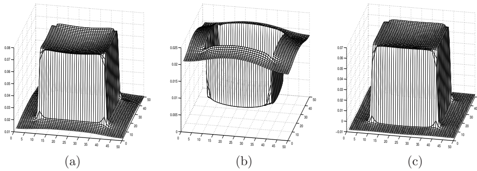
Figure 18: (a) On-Off syncytium (b) Off-On syncytium (c) difference of two syncytia (perceived surface)
