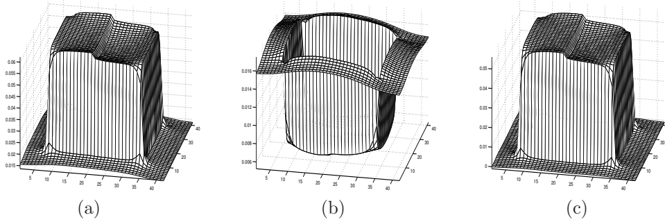
Figure 22: (a) On-Off synctium (steady-state) (b) Off-On synctium (c) On-Off minus Off-On synctia outputs (perceived surface)
