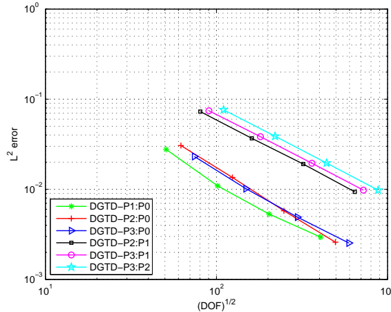
Figure 4.5: Rectangular PEC resonator with one material interface. Numerical convergence of the hp -refinement DGTD- \mathbb{P}_{p_c}:\mathbb{P}_{p_f} method. Non-conforming triangular meshes.
