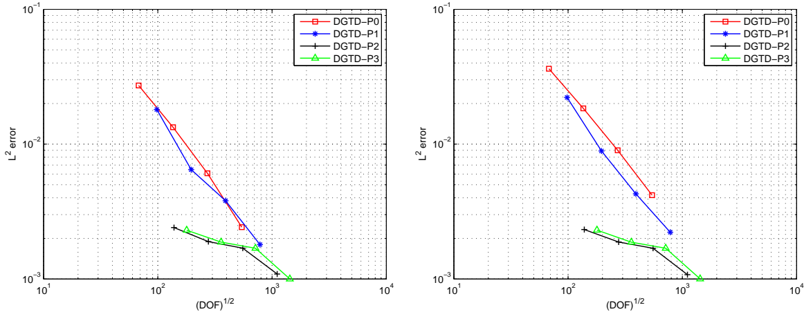
Figure 4.8: Dielectric in a PEC cavity with two material interfaces with \epsilon_2 = 2.25 . Numerical convergence of the h -refinement DGTD\text{-}\mathbb{P}_p method. Conforming (left) and non-conforming (right) triangular meshes.
