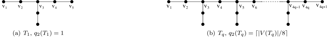
FIGURE 5. Tree T_q , q \geq 1 , with 8q - 1 nodes such that q_2(T_q) = q = \lceil |V(T_q)|/8 \rceil .
