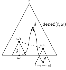
Fig. 2. Given t and \omega_1 , let us suppose that at position \omega the subterm t|_\omega contains a reference to the subterm d (i.e. d = \text{deref}(t, \omega) ). The translation from \omega_1 to \omega_2 corresponds to an update of t|_{\omega_1} as if it was moved to \omega_2 . To maintain the pointers to the referenced terms, the paths stored in t|_{\omega_1} are updated. The result of this operation is the updated subterm t|_{\omega_1} . For example, f(g(-1 \cdot -1), a)_{[1 \rightarrow 2]} = g(-1 \cdot -2) .
