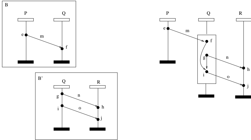
Figure 11: Construction of Future_{B \odot B'}(\bar{m})
