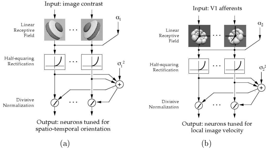
Figure 2.1: Simoncelli and Heeger's model. The V1 and MT cells follow the linear/non-linear pattern with a non-linearity introduced by the shunting inhibition.
