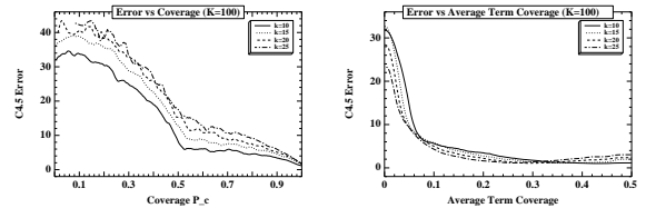
Figure 6. C4.5 Error vs Coverage and Average Term Coverage in k -term DNF languages, for m = 50 , k = 10, 15, 20, 25 , with Gaussian parameter K = 100 .
