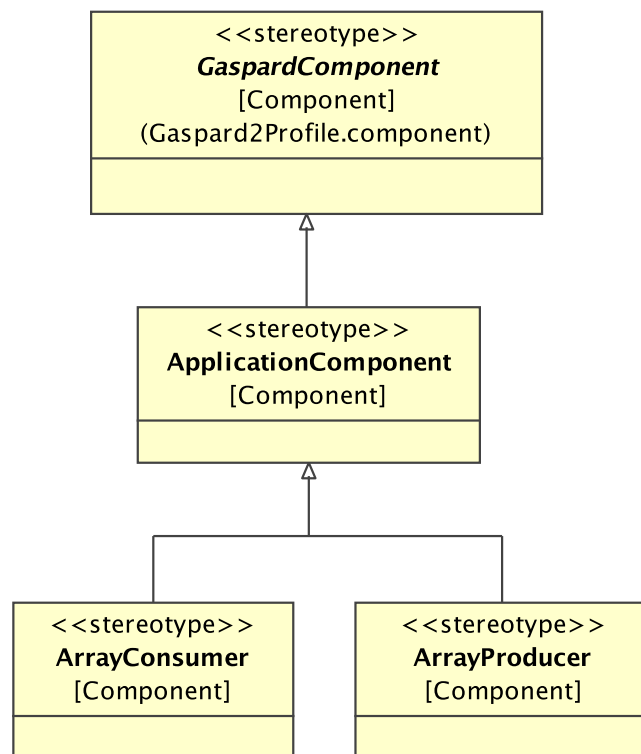
Figure 5.1: Application components
