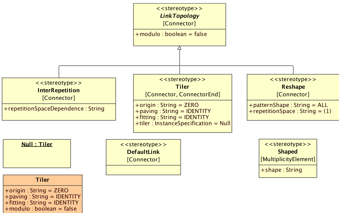
Figure 3.1: Concepts of the factorization package
