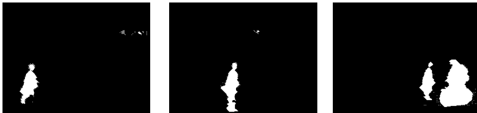
Our method
