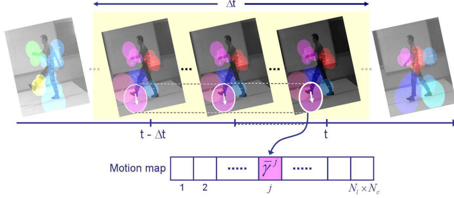
Figure 14: Diagram summarizing the construction of the motion map H_I . A sliding window of width \Delta t is defined. Inside that window, for the j -th cell the mean firing rate \gamma_I^j(t) is calculated. Finally, the motion map is built using the windowed firing rate \bar{\gamma}_I^j(t) of each j -th cell.
