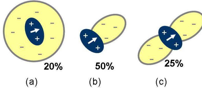
Figure 11: Different geometries of asymmetric center-surround organization in MT cells [66, 65]. (a) Circularly symmetric surrounds. (b) Asymmetric configuration concentrating the suppression at one side of the motion preferred axis. (c) Bilaterally symmetric zones of suppression lying in the motion preferred axis.
