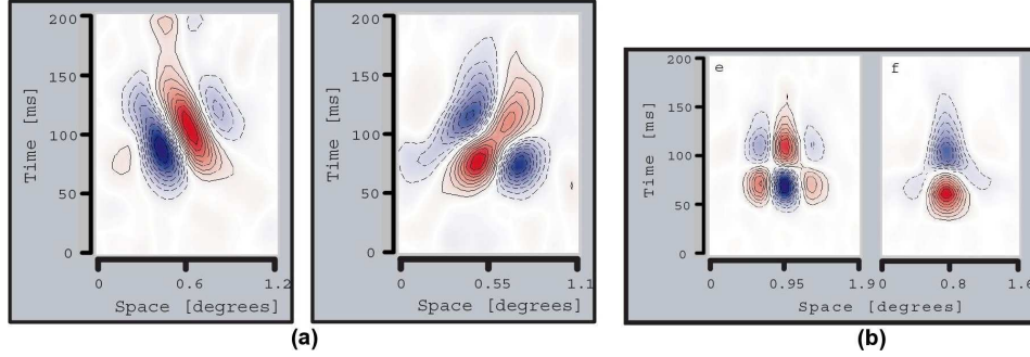
Figure 2: Examples of spatio-temporal receptive fields of V1 cells (from [19]). (a) Spatio-temporal diagrams of two directionally-selective V1 simple cells. (b) Spatio-temporal diagrams of two biphasic V1 simple cells with short latencies.
