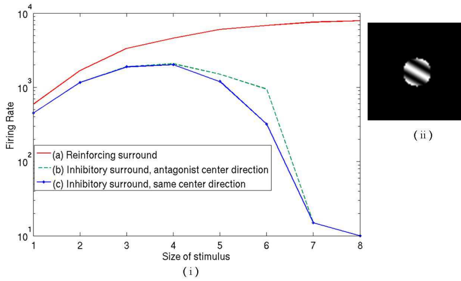
Figure 13: Graph with the firing rates measured for the three different receptive fields modeled for MT cells (Figure 12). The stimulus consisted in a circle of variable radius with a drifting grating inside (ii). The effect of vary the radius of the stimulus in the firing rate of the cell is graphed in (i). Each curve corresponds to the receptive fields (a), (b) and (c) defined in Figure 12. The motion direction tuning of the center of each MT cell corresponds to the orthogonal direction of the drifting grating. Here it is possible to see the no-reaction for wide-field motion in the case of antagonistic surrounds cells.
