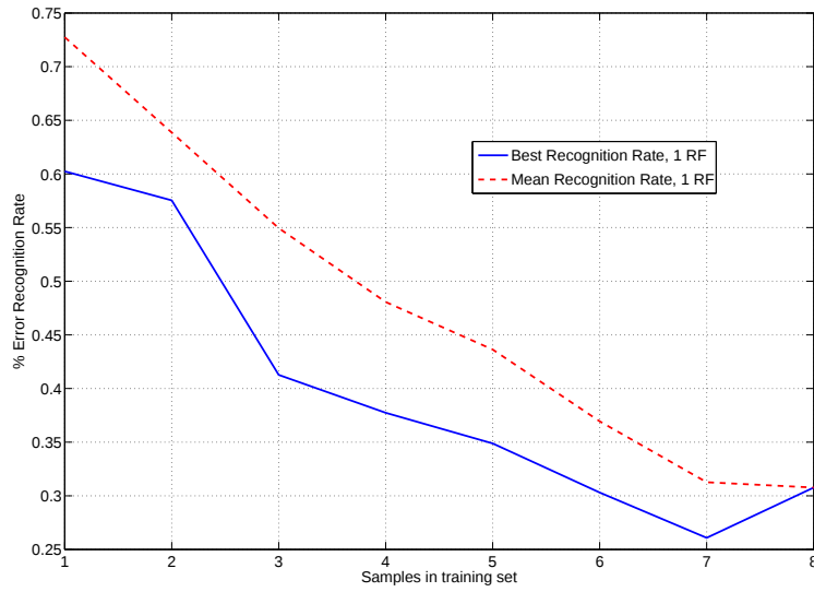
Figure 17: Recognition error rate obtained for the ground truth configuration and the Weizmann database. In this case just one receptive field ( reinforcing ) were used.
