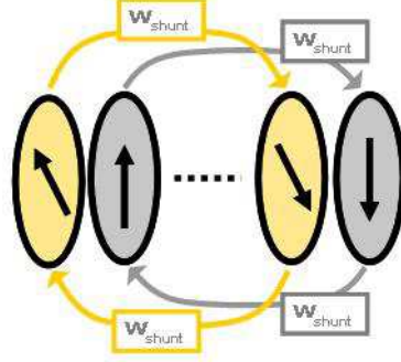
Figure 7: Inhibitory interactions between cells of the same column. The interaction occurs within cells oriented in opposite directions. The first cell spiking sends an inhibitory signal to the cell in the same column tuned to the opposite motion direction.
