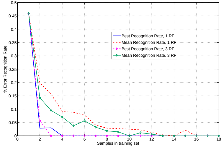
Figure 18: Recognition error rate obtained for Giese database using the three different receptive fields described in Figure 12. It is possible to see an improvement in the recognition error rates in comparison with the case of just one receptive field (Figure 16).
