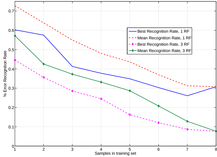
Figure 19: Recognition error rate obtained for Weizmann database using the three different receptive fields described in Figure 12. The improvement obtained with the approach of the three receptive fields instead only one is considerably.
