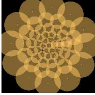
Figure 9: Sample of log-polar architecture used for a MT layer. The cell distribution law is divided into two zones, a homogeneous distribution in the center with a certain radius and then a periphery where the density of cells decays with the eccentricity.
