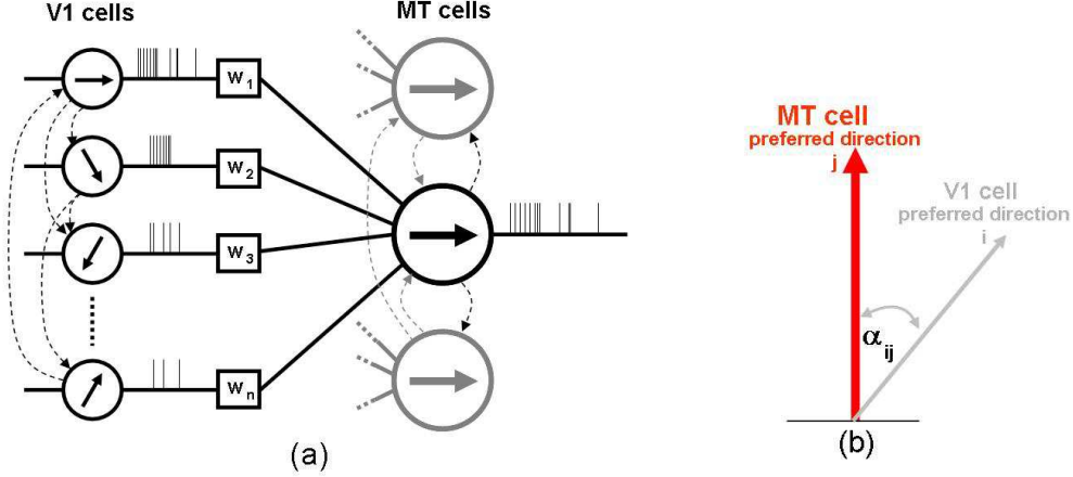
Figure 10: Architecture of the spiking neural network to model MT. Each MT cell receives as input the afferent V1 cells (a). The connection weights between V1 and MT cells are modulated by the cosine of the angle \alpha between the preferred direction of MT cell and the preferred direction of V1 cell (b).
