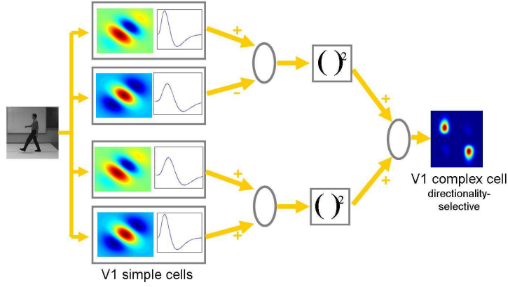
Figure 5: Diagram with the procedure described in [1] to create a V1 complex cell starting from V1 simple cells. At the output a directionally-selective cell is obtained.
