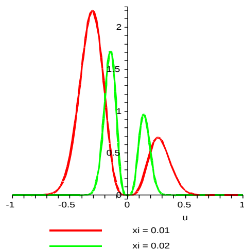
Figure 20: Curves showing the behaviour of \tilde{g}^x(\xi) for two different frequencies f (0.01 and 0.02). In the graphs it is possible to see the maximal value reached along the negative spatial frequencies.
