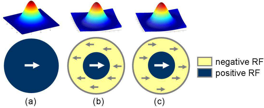
Figure 12: Center-surround interactions modeled in the MT cells. The reinforcing surround (a) is modeled through a gaussian. The two receptive fields with inhibitory surround (b), (c) are modeled with a Difference-of-Gaussians. The cells with inhibitory surround have either antagonistic direction tuning between the center and surround or the same direction tuning.
