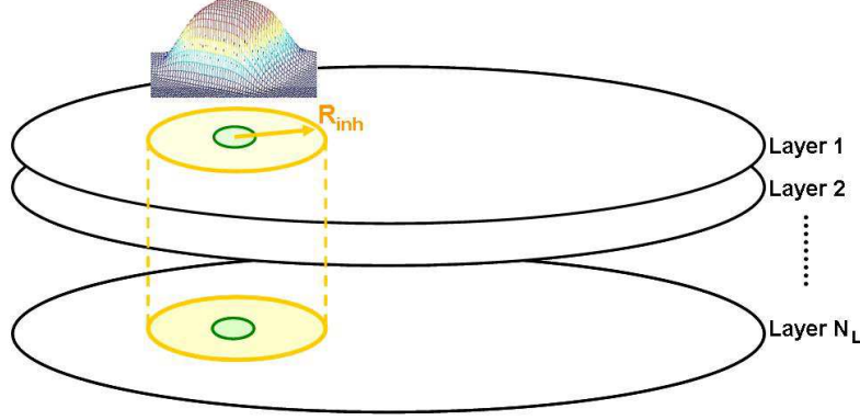
Figure 8: Extra-column inhibition mechanism. Each cell has a radius of action R_{inh} from where it polls information to adjust its own activation level.
