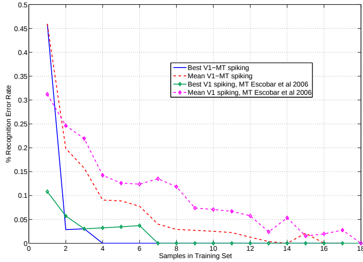
Figure 16: Recognition error rate obtained for the ground truth configuration and the Giese database. In this case just one receptive field ( reinforcing ) were used. It is also included the comparison with the results obtained in [22].
