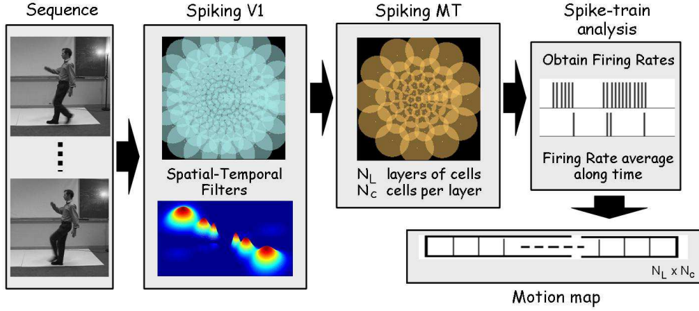
Figure 1: Block diagram showing the different steps of our approach from the input image sequence as stimulus until the motion map encoding the pattern motion. The directional-selectivity filters are applied over each frame of the input sequence in a log-polar distribution grid obtaining spike trains as V1 output. These spike train feed the spiking MT which integrates the information in space and time. The motion map is constructed calculating the mean firing rates of MT cells along the length in time of the input sequence. The motion map has a length of N_L \times N_c elements, where N_L is the number of MT layers of cells and N_c is the number of MT cells per layer.
