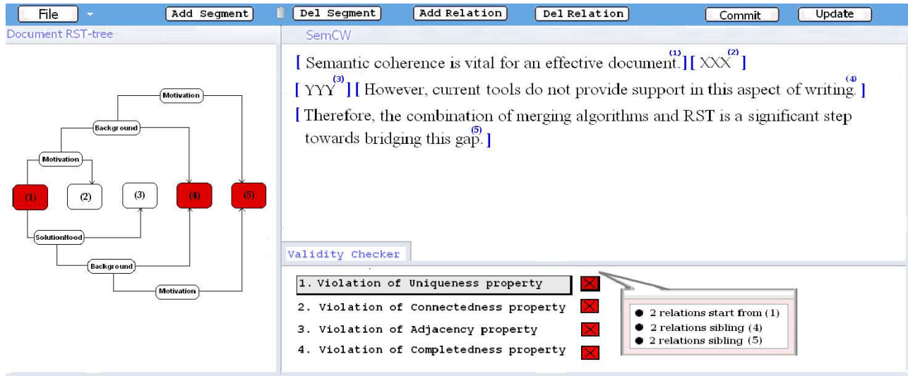
Figure 10: The validity checker
