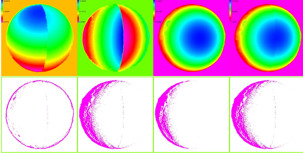
Figure 5: Top: the recovered u, v, d, d' maps for the ball example ( -7 < u < 4 , -4 < v < 4 , -113 < d < 1 , -115 < d' < 2 ). Notice the vertical discontinuity in d' , due to the fact that the reference coordinates are those of the left image at time t . Bottom: the occlusion maps for the data terms corresponding to left flow, right flow, disparity at t and disparity at t + 1 .
