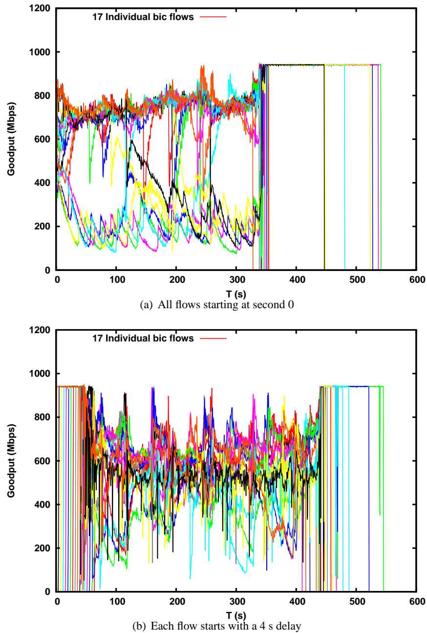
Figure 3: Influence of flows' inter-arrival on BIC: 1.7 congestion level (17 flows), 19.8 ms RTT
