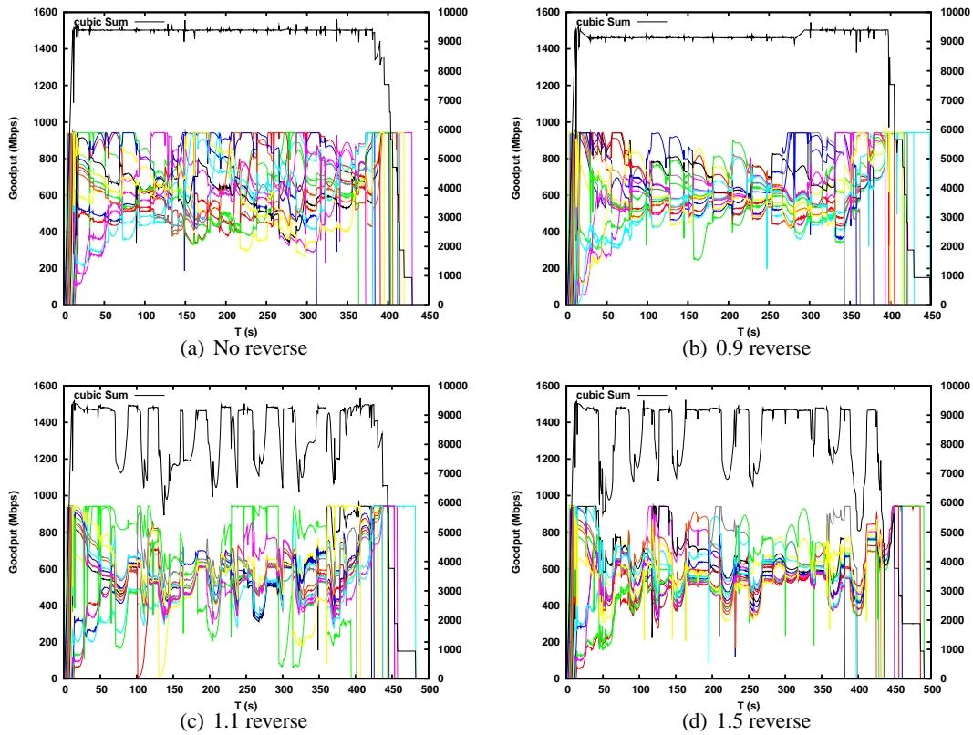
Figure 17: Effect of various reverse traffic level on a fixed congestion level for CUBIC, 19.8 ms RTT
