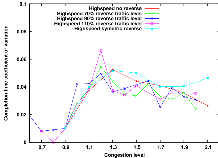
Figure 21: Evolution of the completion time coefficient of variation for different reverse traffic level for Highspeed, 19.8 ms RTT
