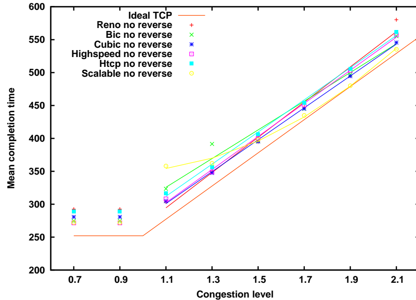
Figure 5: Impact of congestion level on the mean completion time for all TCP variants
