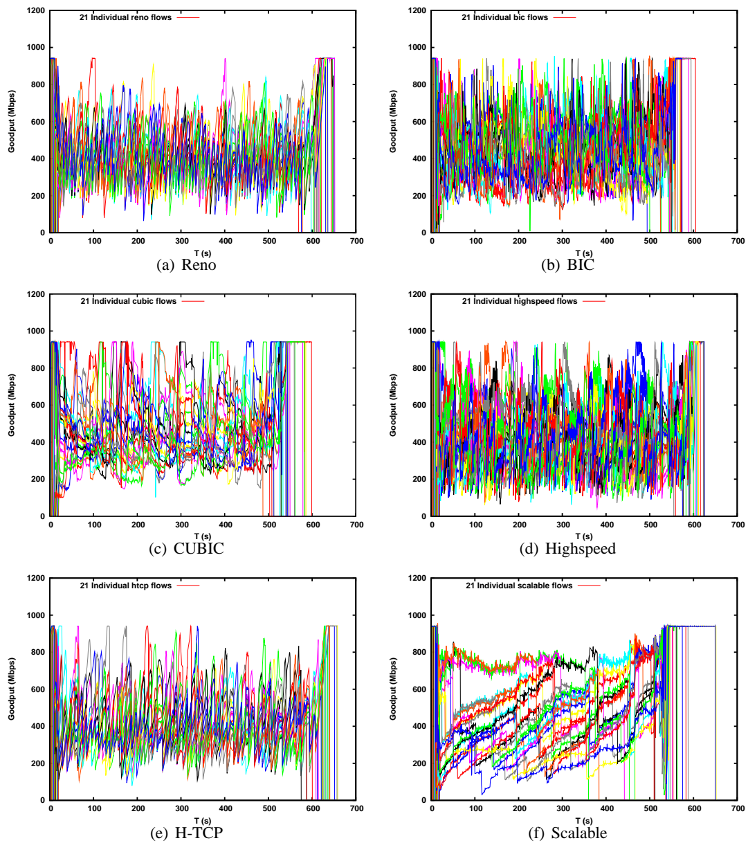
Figure 4: Impact of a high congestion level: 2.1 congestion level (21 flows), 19.8 ms RTT, on CUBIC and Scalable
