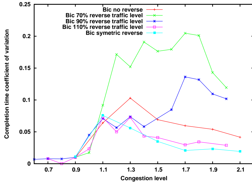
Figure 19: Evolution of the completion time coefficient of variation for different reverse traffic level for BIC, 19.8 ms RTT
