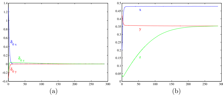
Figure 3: Proportional control \mathbf{v} = k_{\delta}\boldsymbol{\delta} : time evolution of the image feature \boldsymbol{\delta}_0 = \mathbf{R}\boldsymbol{\delta} (a), and of the pose \boldsymbol{\xi}_0 (b).
