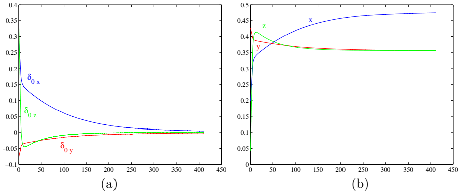
Figure 8: GAS control design \mathbf{v} = k_M \mathbf{M} \delta_{\mathbf{f}} : time evolution of the image feature \delta_0 = \mathbf{R} \delta_{\mathbf{f}} (a), and of the pose \xi_0 (b).
