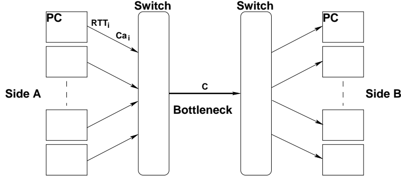
Figure 2: Experiment topology
