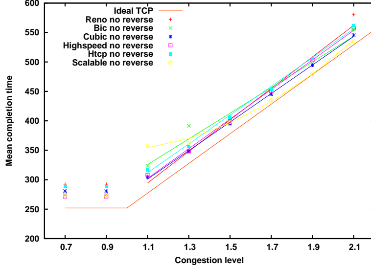
Figure 8: Impact of congestion level on the mean completion time on TCP variants, 19.8 ms RTT
