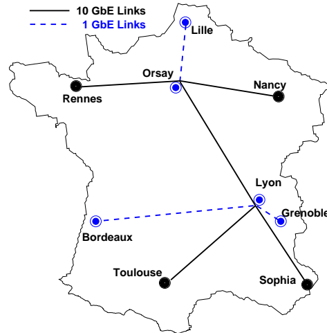
Figure 1: Grid'5000 backbone
