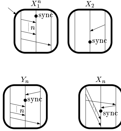
Figure 5: Two MSCs Y^n, X^n in the monitored product of X_1^n and X_2
