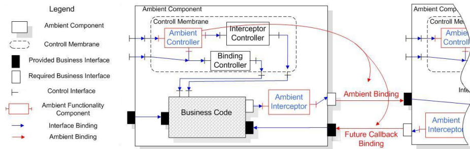
Fig. 2. Ambient Component
