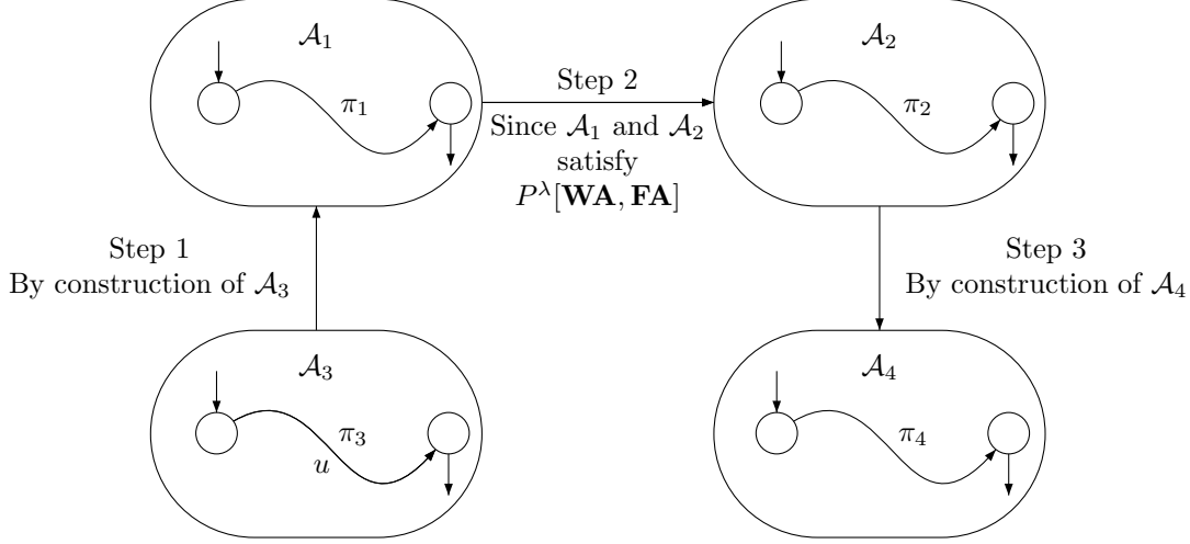
Figure 4: Proof of Proposition 10, part 1.
