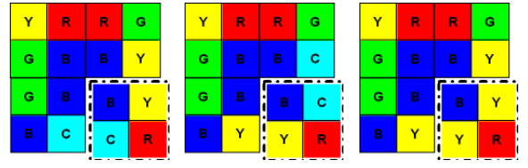
Figure 3: The cases why the two additional tiles in Figure 2(c) are required.
