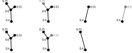
Figure 5: Deletion of edges whose weight is lower than or equal to t_2 = 0.15 . Top: without weight ordering. Bottom: with weight ordering.
