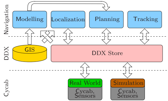
Fig. 1. Functional view of the navigation architecture.
