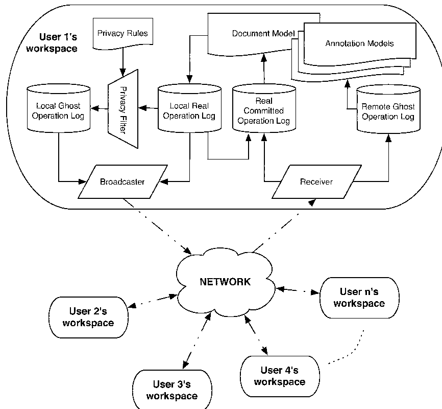
Figure 3: Gasper Architecture
