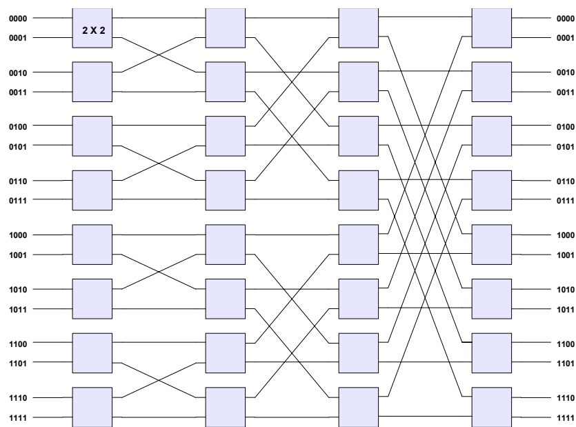
Figure 23: A Reverse Butterfly (16,2) Network
