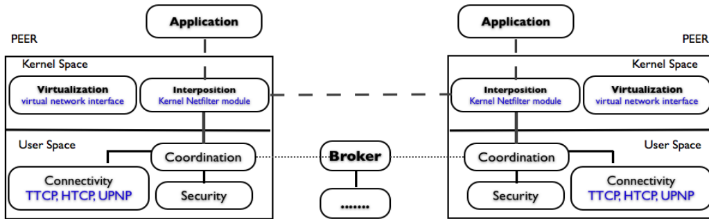
FIG. 2 – PVC architecture
