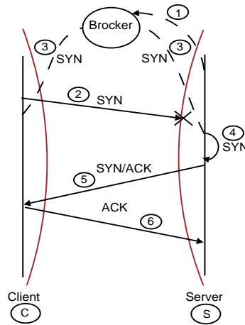
FIG. 3 – Traversing-TCP
