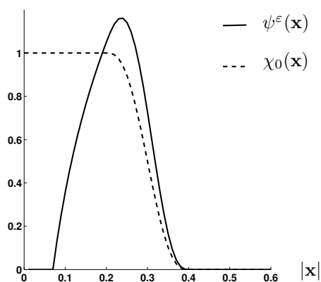
Figure 5: Graph of the additional function \psi^\varepsilon
