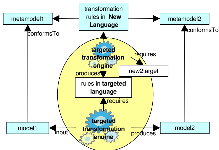
Figure 7: New Transformation Language executed on top of existing transformation engine.
