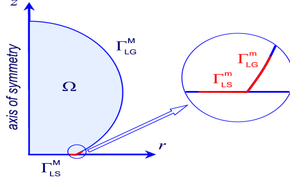
Figure 3. A droplet put down on a solid surface.
