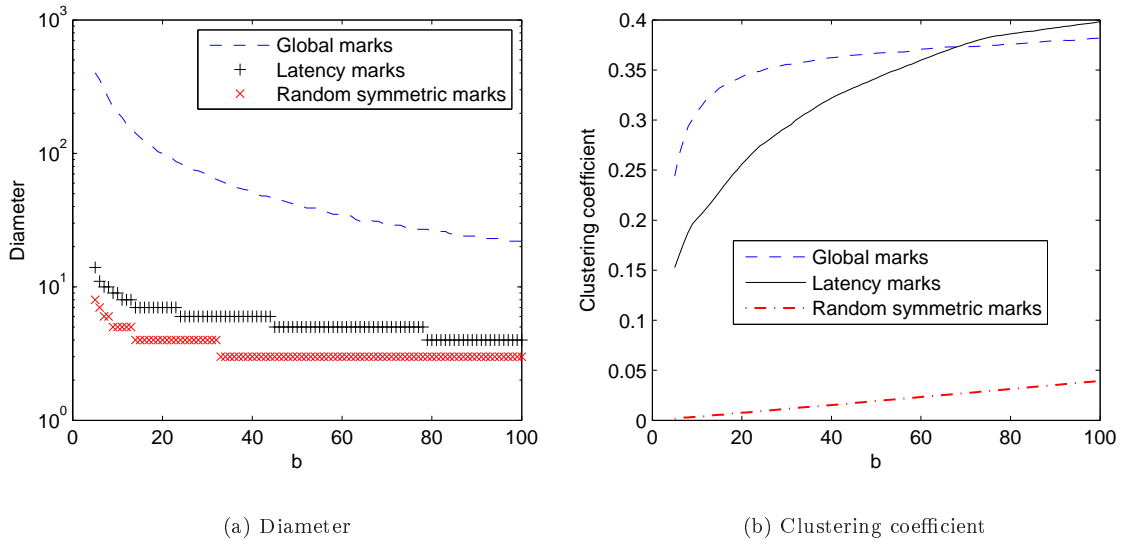
Figure 1: Diameter and clustering coefficient of latency, random symmetric and global marks (2500 nodes) stable configurations. Global marks use an underlying Erdős-Rényi \mathcal{G}(2500, 0.5) acceptance graph.
