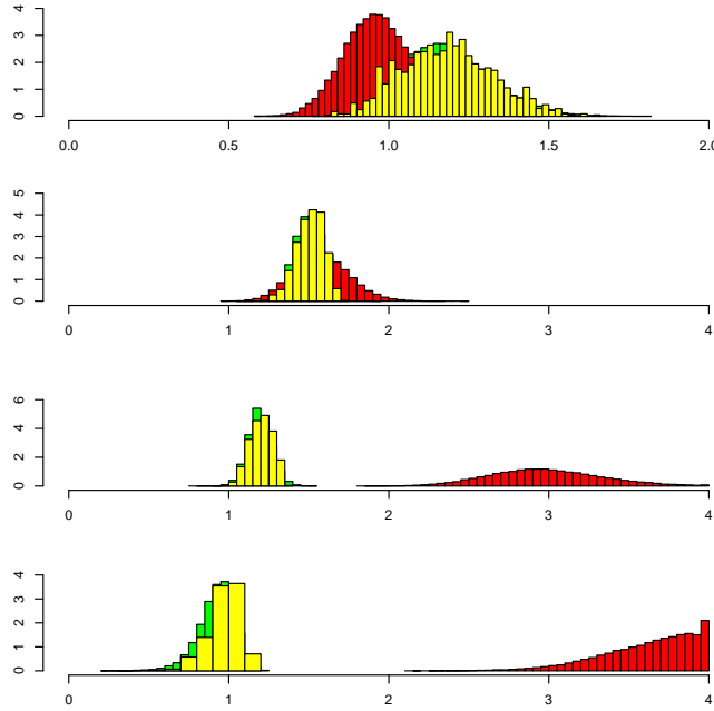
Figure 10: Comparison of the approximations to the posterior distribution of \beta based on the pseudo (red), the path (green) and the perfect (yellow) schemes for Ripley’s benchmark and k = 1, 10, 70, 125 , for 20,000 iterations and 10,000 burn-in.
