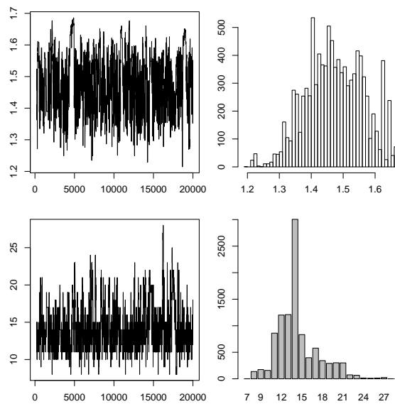
Figure 7: Output of a random walk Metropolis–Hastings algorithm based on the perfect sampling elimination of the normalising constant for a plug-in estimate (\hat{k}, \hat{\beta}) = (13, 1.45) and 20,000 iterations, with a 10,000 burn-in stage and \tau^2 = .05 , r = 3 : ( top ) sequence and marginal histogram for \beta and ( bottom ) sequence and marginal barplot for k .
