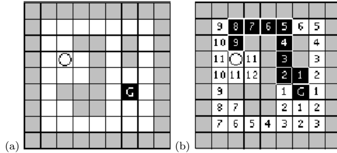
Fig. 1. WaveFront algorithm: initial environment state and result of the construction
