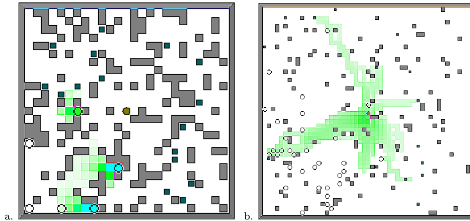
Fig. 11. Foraging with ants that drop pheromones and use “compass”-like information to return to their nest situated in the center. a) obstacle density of 30% generates cavities where agents freeze. b) obstacle density of 5% does not interfere with foraging (50 x 50 env., 50 ants, 20 sources)
