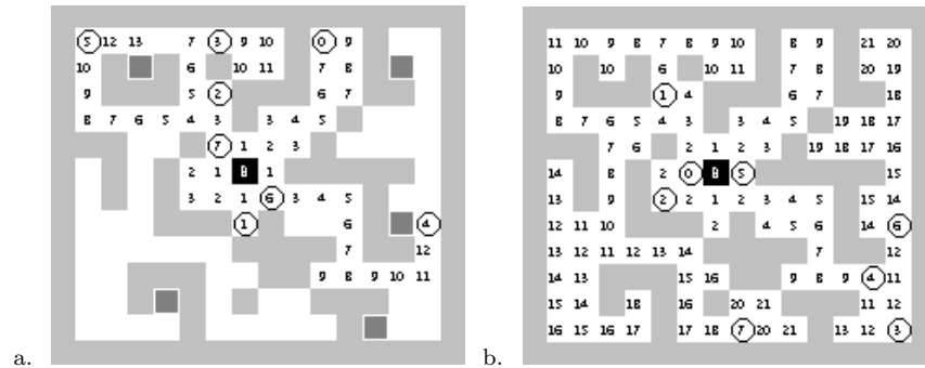
Fig. 3. Foraging with eight marking agents in a little maze (a) after 18 iterations (b) final state
