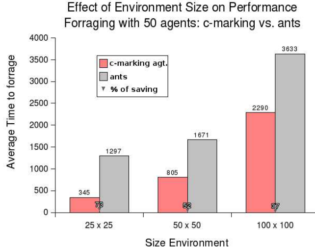
Fig. 9. Comparison of the performance of the markings model with the ant-model as the size of environment is varied ( Setup (3) ): 50 agents, 5% of obstacles, 20 resources of 2000 units).
