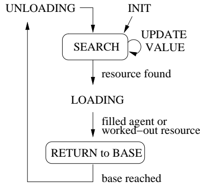
Fig. 4. Behaviour of a marking agent in foraging
