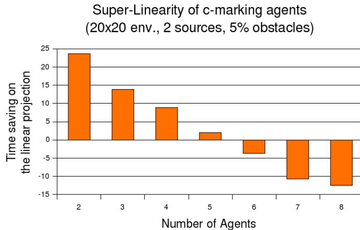
Fig. 8. Difference in projected and actual number of iterations required, on average, to achieve foraging in Setup (2) - when varying number of agents - (Table II)
