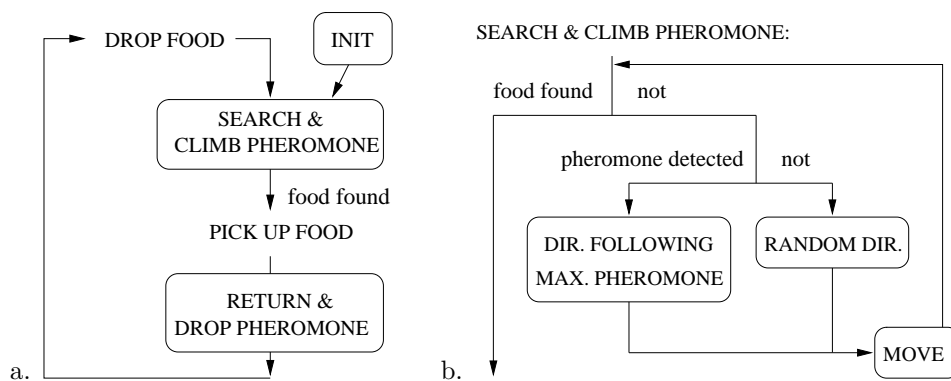
Fig. 10. The ant model: (a) global ant behavior (b) details into task Search & Climb pheromone
