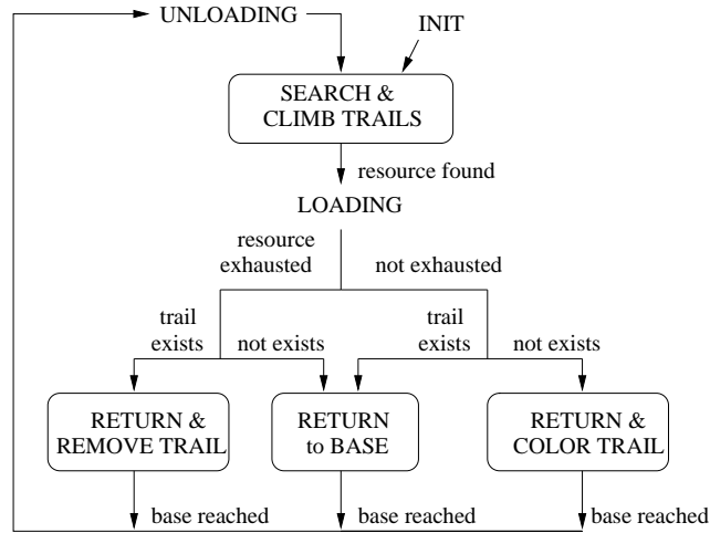
Fig. 5. c-marking agents that colour paths between sources and the base
