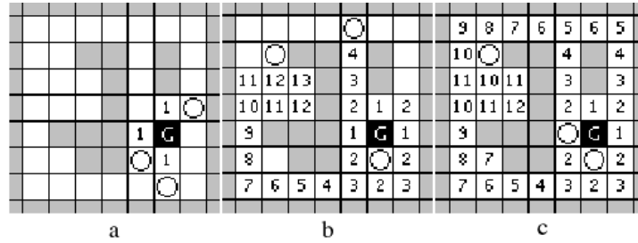
Fig. 2. Collective construction of the potential field with 3 agents (steps 2, 17 and 65)
