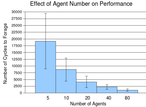
Fig. 7. Performance of c-marking agents in Setup (1) (Table I)
