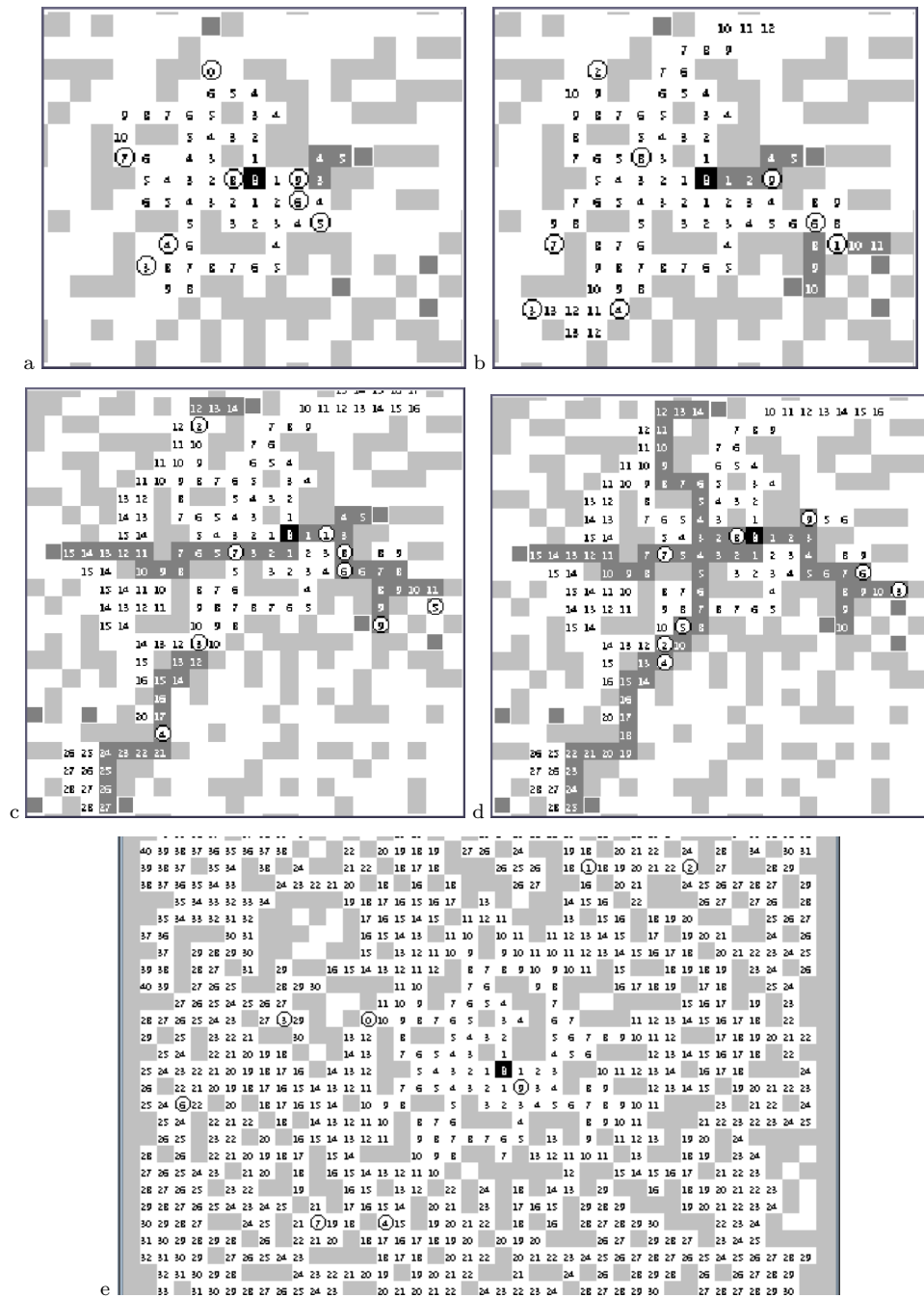
Fig. 6. Resolution of the foraging problem with 10 c-marking agents (with Setup 1 ). Trails are represented in dark grey colour. Snapshots at step 11, 21, 53, 76, 1200.
