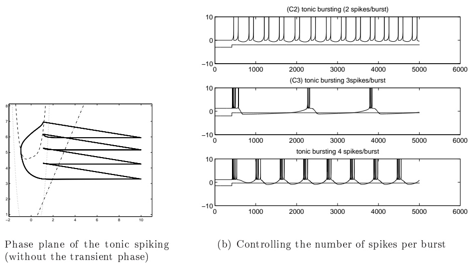
(a) Phase plane of the tonic spiking (without the transient phase) (b) Controlling the number of spikes per burst Figure 7: Tonic bursting: phase plane trajectory. The black curve is the v nullcline at the initial time. It is shifted to the red one when applying a constant input current. The new dynamical system has no fixed point. We can see the multiple spike limit cycle here.
