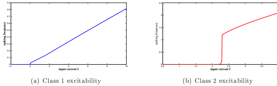
Figure 8: Spiking frequency vs input current I for different choices of b . These curves have been obtained running simulations for different values of the input current, computing the frequency of the emitted spikes in a time range T = 10000 .
