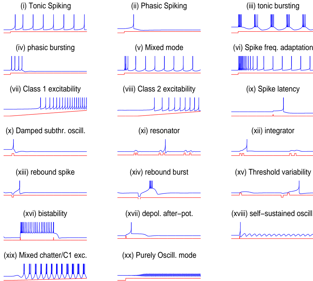
Figure 5: Different remarkable neuro-computational interesting behaviors of the neuron model (4.1) with the reset condition (4.2), for different choices of the parameters (a, b, I, v_r, d) . The blue curve represents the membrane potential v and the red one the input current I (see annex ?? for the numerical values of each simulations).
