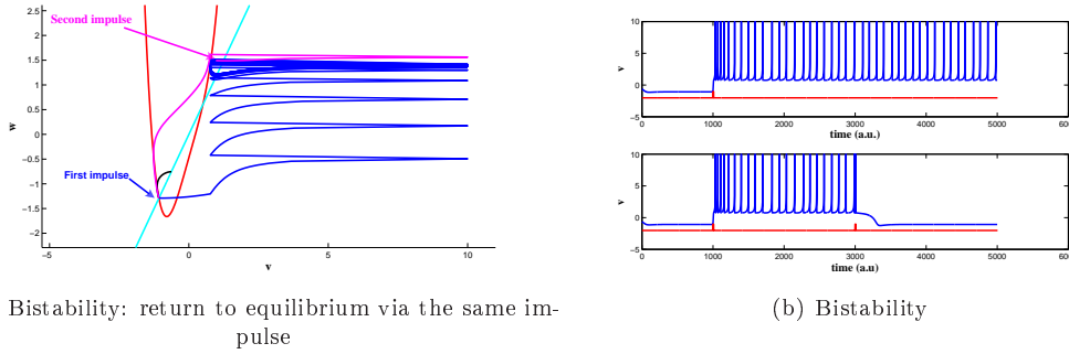
Figure 9: Bistability phenomenon: The first impulse induces a self-sustained tonic spiking behavior while the system has a stable fixed point. The second impulse perturbs this regular spiking behavior and the system falls in the attraction basin of the stable fixed point.
