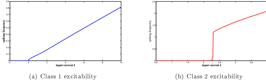
Figure 7: Spiking frequency vs input current I for different choices of b . These curves have been obtained from running simulations for different values of the input current, computing the frequency of the emitted spikes in a time range T = 10000 .
