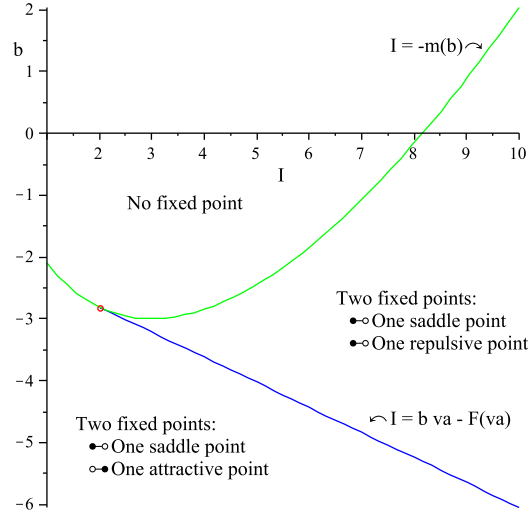
Figure 1: Number of fixed points and their stability in the plane (I, b) , for the exponential adaptive model.
