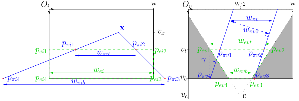
Fig. 2. Principle of the IPM transformation: the road boundaries converge to the DVP x in \mathcal{R}_i and appear parallel in \mathcal{R}_v . The intersections of the image boundaries and the road borders with the two parallel lines \mathbf{l}_b and \mathbf{l}_t respectively generate the quadruplets \{\mathbf{p}_{e1}, \mathbf{p}_{e2}, \mathbf{p}_{e3}, \mathbf{p}_{e4}\} and \{\mathbf{p}_{\pi 1}, \mathbf{p}_{\pi 2}, \mathbf{p}_{\pi 3}, \mathbf{p}_{\pi 4}\} .
