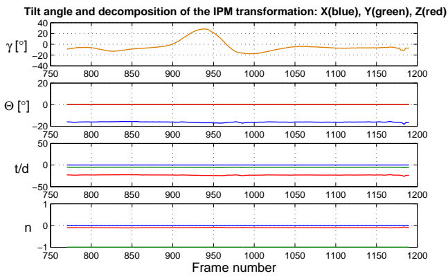
Fig. 6. Orientation of the camera (brown) and decomposition of the H_{prvi} homography along the Antibes sequence. The numerical values are given up to a scale factor due to the pixels of the IPM image are not squared and the camera is not calibrated ( d = 1m ).
