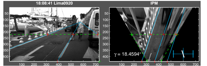
Fig. 3. The IPM transformation is computed thanks to the intersections of the first and the third blue medians of the road boundaries with the green \mathbf{l}_b and \mathbf{l}_t lines. The second median is shown for convenience.
