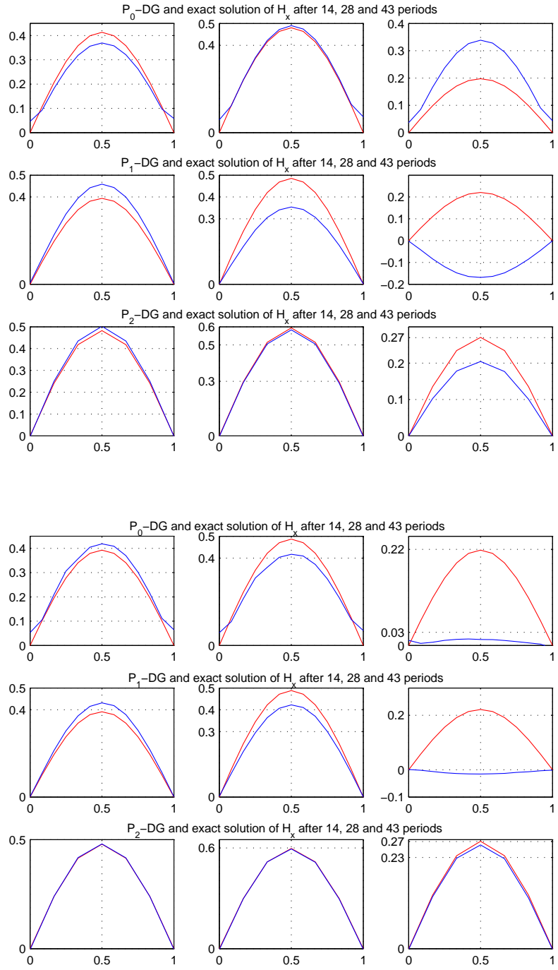
Figure 4.14: 1D distributions of H_x : exact (in blue) and \mathbb{P}_p -DGTD solutions ( p \leq 2 ), regular (top) and irregular (bottom) meshes.
