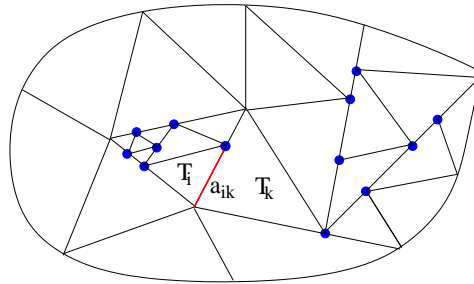
Figure 2.1: Irregular mesh with blue hanging nodes.
