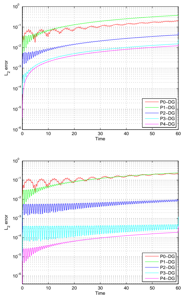
Figure 4.13: Time evolution of the L^2 error: \mathbb{P}_p -DGTD schemes. Logarithmic scale on the y -axis. Regular (top) and irregular (bottom) meshes.
